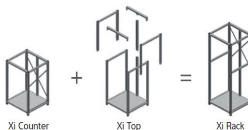
Xi Rack Basic & extension (sample picture)
