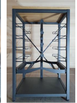
6. 4 Gummipuffer aufkleben und Platte fixieren Montage der Flaschenauflagen laut Folgeseite Xi Counter Anbau direkt an Basis anbauen Optionale LED Beleuchtung laut separater Anleitung nun anbringen 6. Mounting of 4 rubber pads and table plate Mounting of bottle rests as described on following page, Xi Counter Extension can be added directly at Counter Basic Install now optional LED lighting according to separate manual
