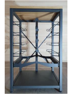
6. 4 Gummipuffer aufkleben und Platte fixieren Montage der Flaschenauflagen laut Folgeseite Xi Counter Anbau direkt an Basis anbauen 6. Mounting of 4 rubber pads and table plate Mounting of bottle rests as described on following page, Xi Counter Extension can be added directly at Counter Basic
